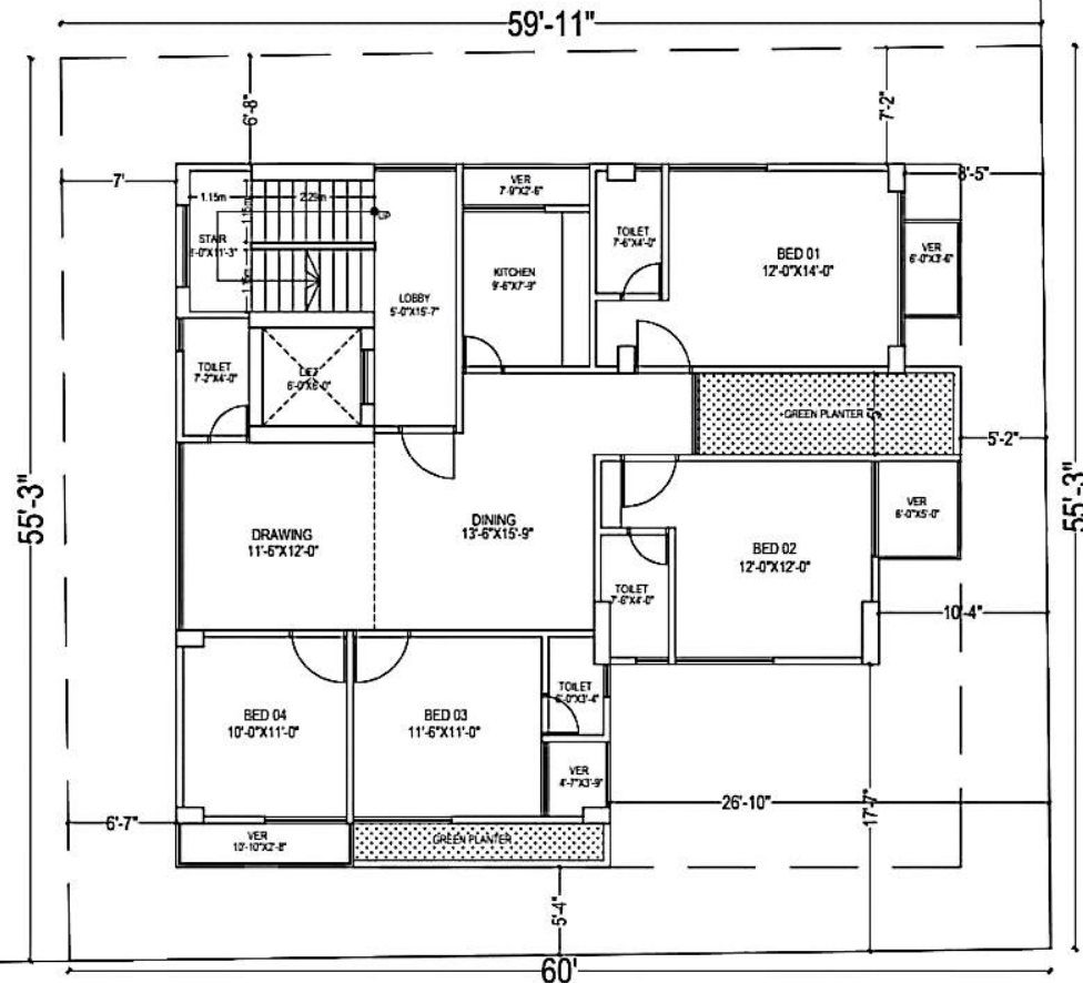
TYPICAL FLOOR PLAN - 1620.27 sq ft SCALE : FIT TO SCALE
